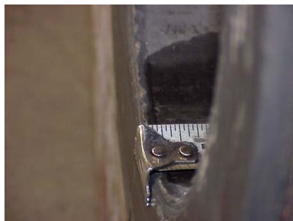
Figure 3-11: Liner with badly coined face, probably due to insufficient contact surface between die and liner face. (Photo courtesy of Lake Park Tool)
